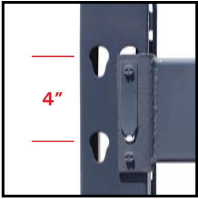
Beams adjustable every 4"
