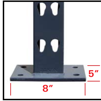
5" x 8" x 3/8" seismic base plates
